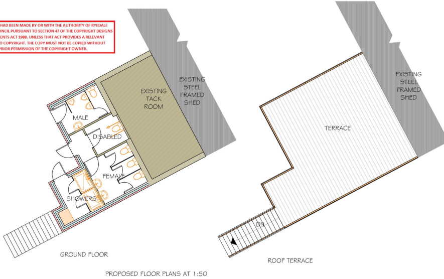
PROPOSED FLOOR PLANS AT 1:50
