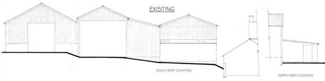
EXISTING & PROPOSED ELEVATIONS AT 1:100
